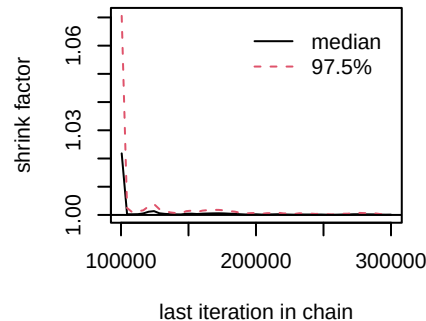
d.I.DHFRi
